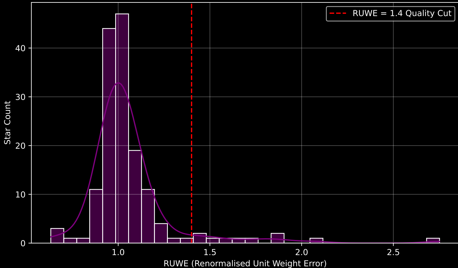
GAPOGEE DR17 Field [006+04-O] RUWE Distribution (n= 153)
