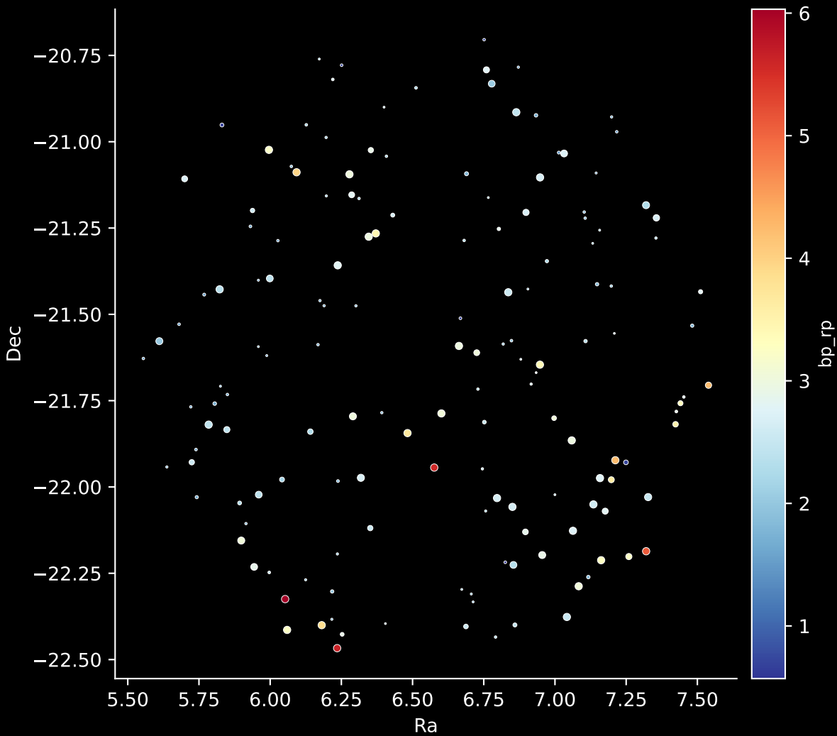
APOGEE DR17 Field: [006+04-O] Stars: 154
