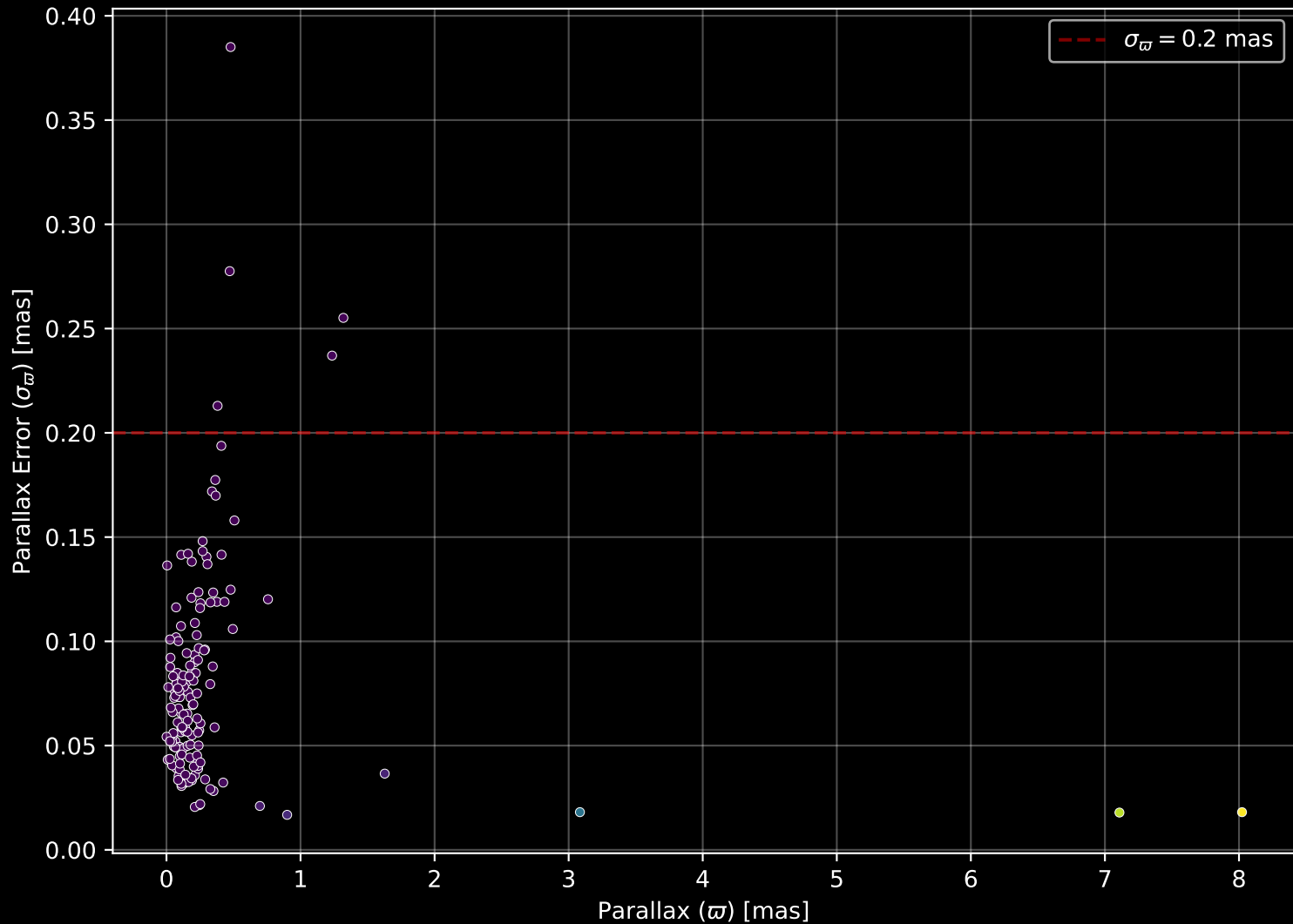
APOGEE DR17 Field: [006+04-O] Parallax Quality (n= 154)
