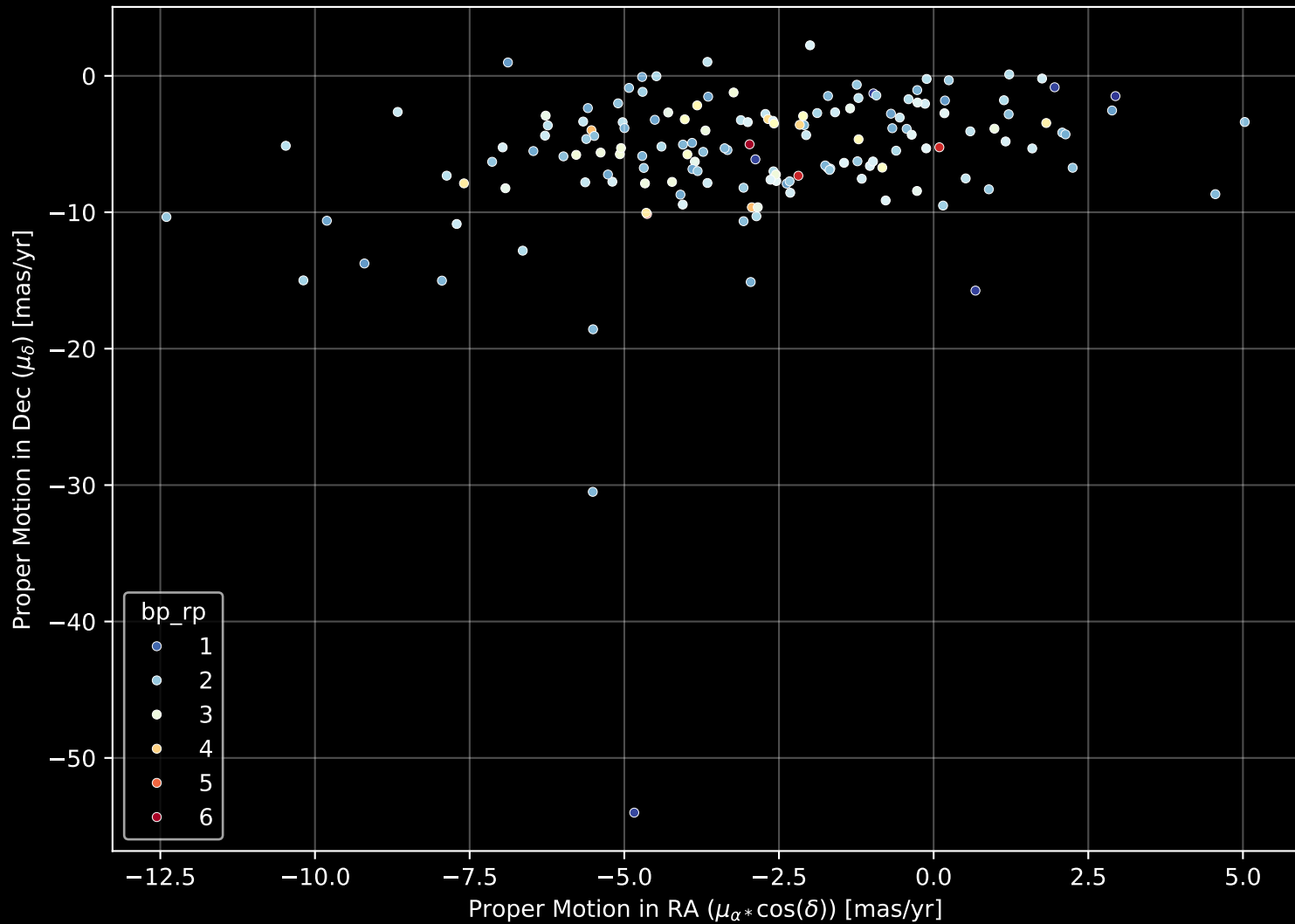
APOGEE DR17 Field: [006+04-O] Proper Motion Diagram (n= 154)
