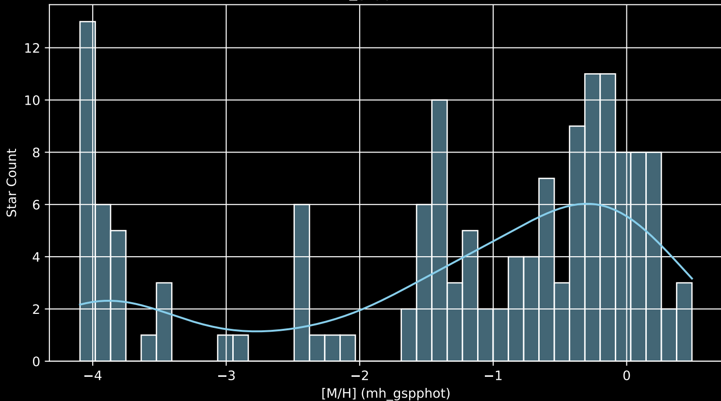
APOGEE DR17 Field: [006+04-O [M/H] (mh_gspphot) (n= 147)
