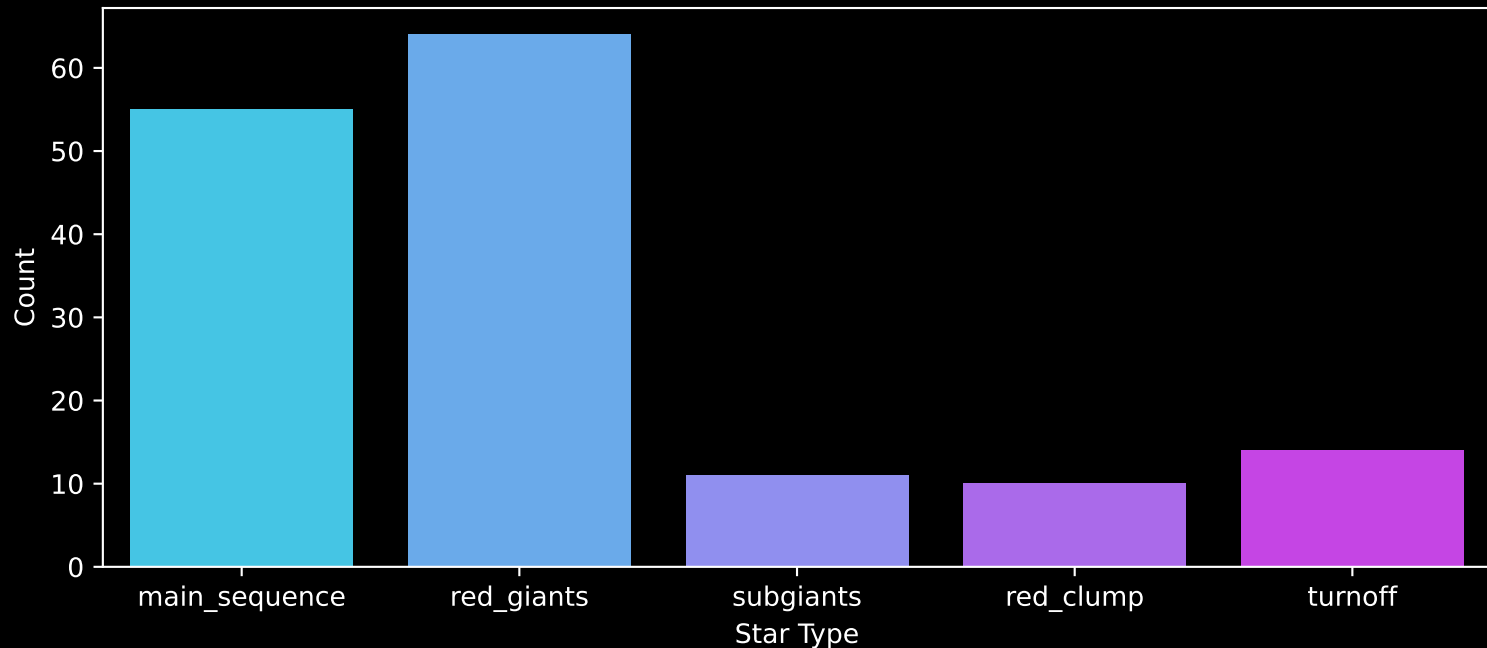
APOGEE DR17 Field: [006+04-O] Count plot of Star Type
